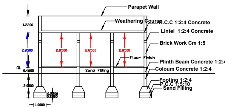
Section Section - AA
