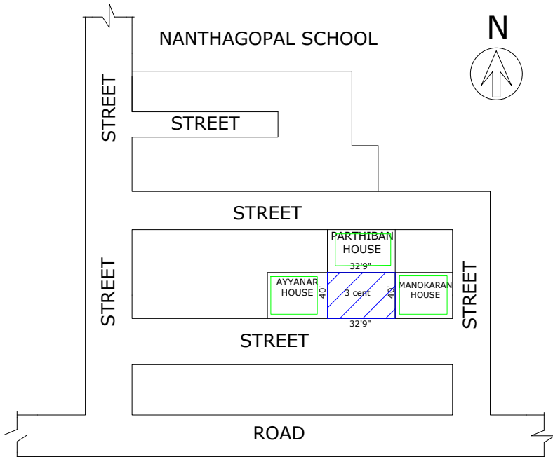
TOPO PLAN
