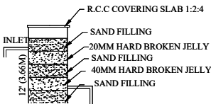
RAIN WATER HARVESTING
