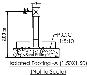
FOUNDATION DETAIL - A
