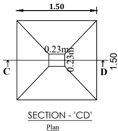
SECTION - 'CD'
