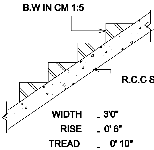
STAIR DETAILS
