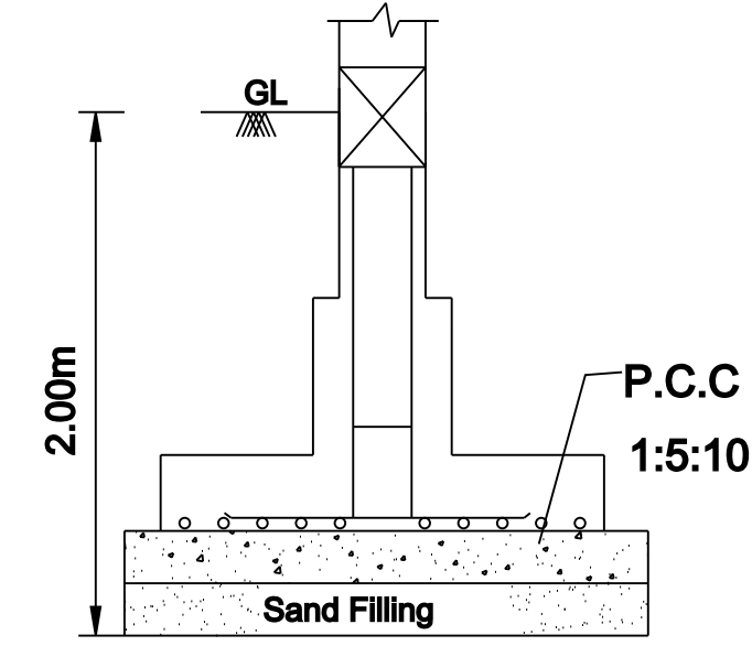
FOUNDATION DETAIL
