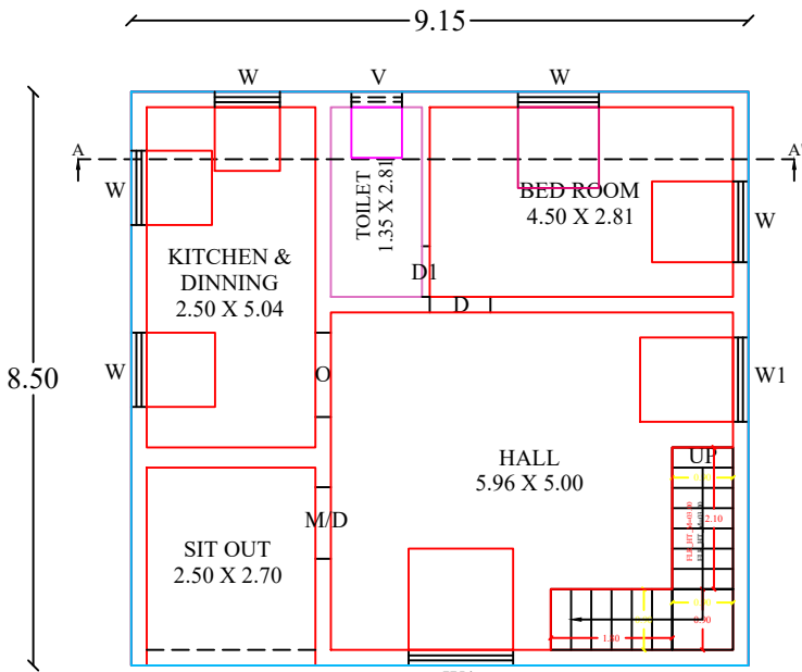
GROUND FLOOR PLAN (NORTH FACING)
