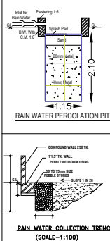
RAIN WATER COLLECTION TRENCH (SCALE-1:100)
