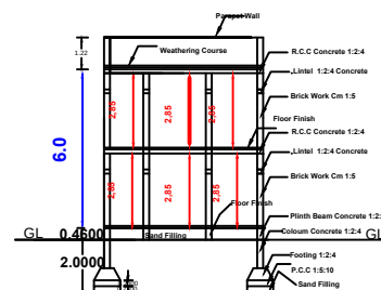
Section Section - AA
