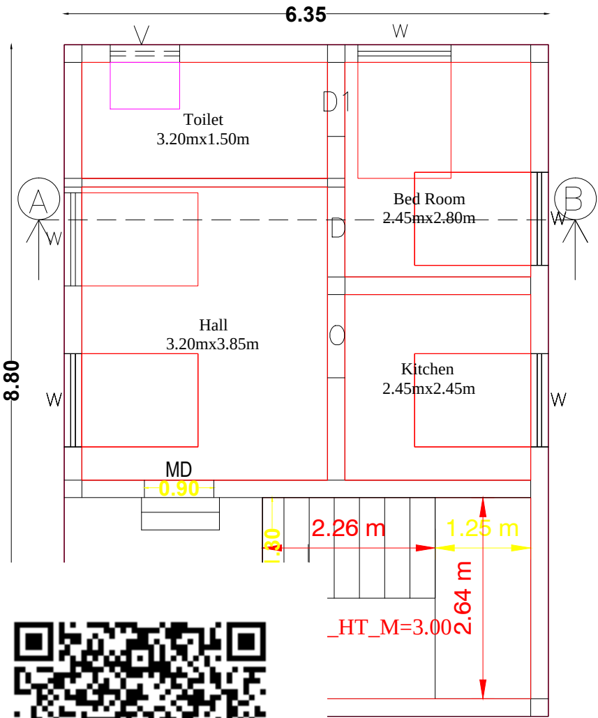
GROUND FLOOR
