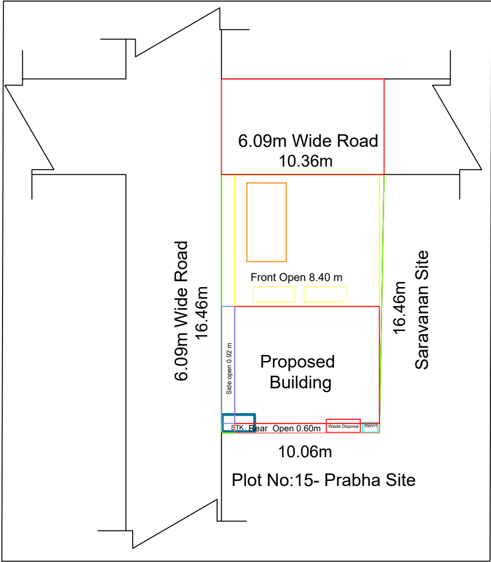
Site Plan
