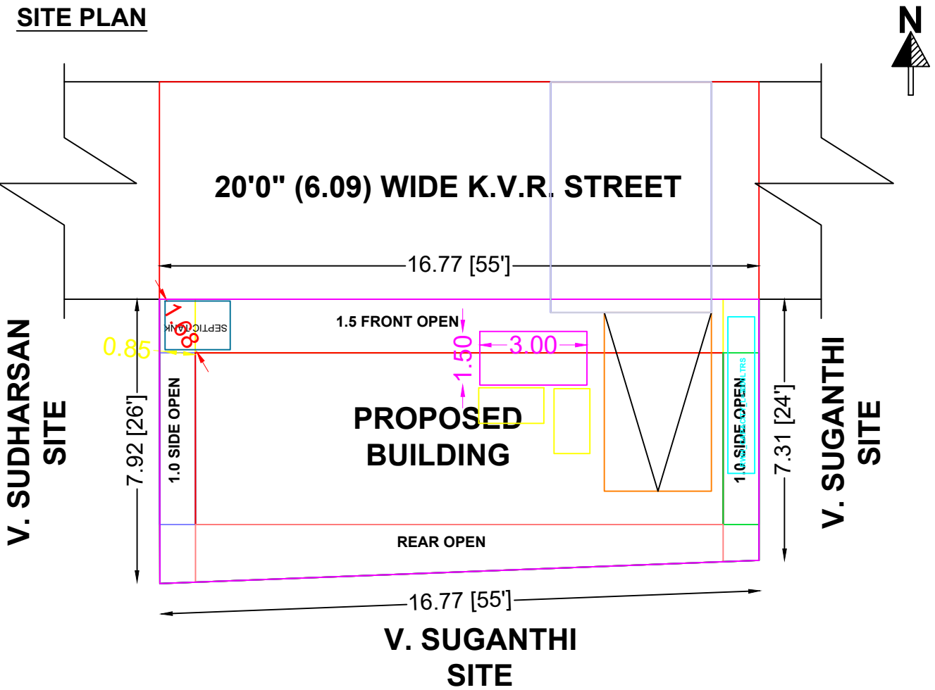
SITE PLAN
