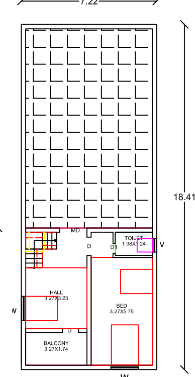
PRO. FIRST FLOOR PLAN
