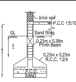
FOUNDATION DETAILS
