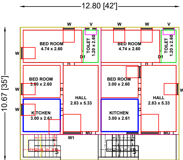
GROUND FLOOR PLAN (EAST FACING)
