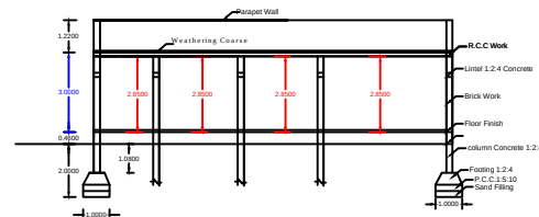
SECTION SECTION - AB
