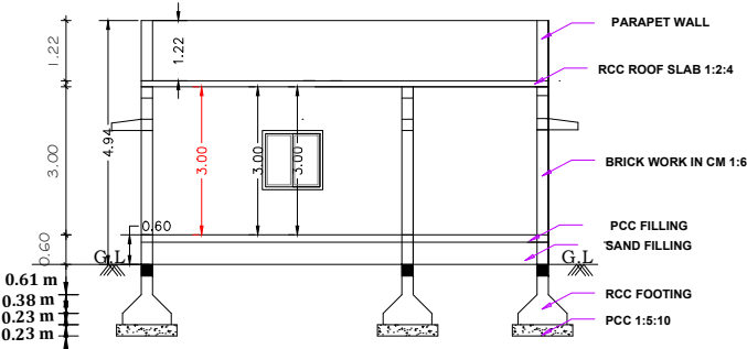
SECTION "A-B"
