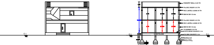
Proposed Additional Ground Floor And Existing First Floor Front Elevation
