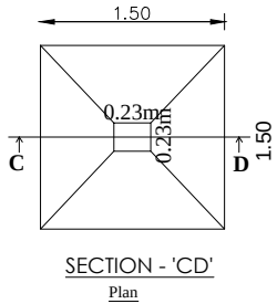
SECTION - 'CD' Plan
