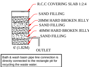
Waste Water Recycle Unit Not To Scale
