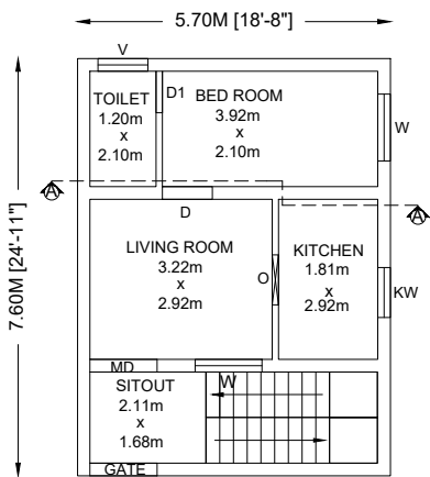
GROUND FLOOR PLAN (NORTH FACING )
