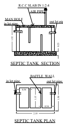
SEPTIC TANK PLAN
