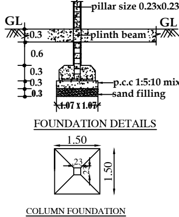
COLUMN FOUNDATION
