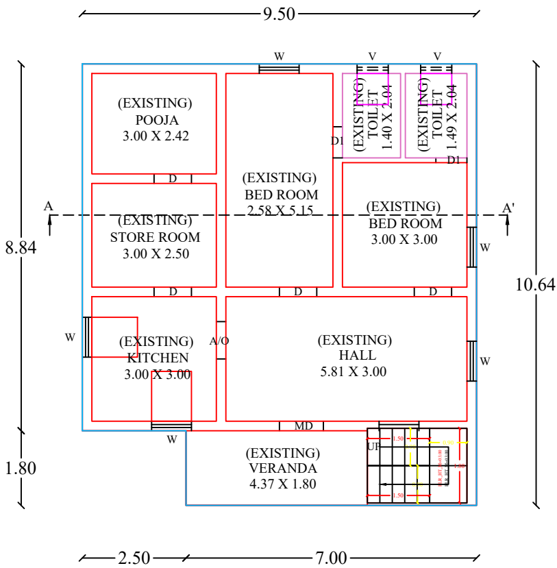
GROUND FLOOR PLAN (EXISTING BUILDING) (EAST FACING)
