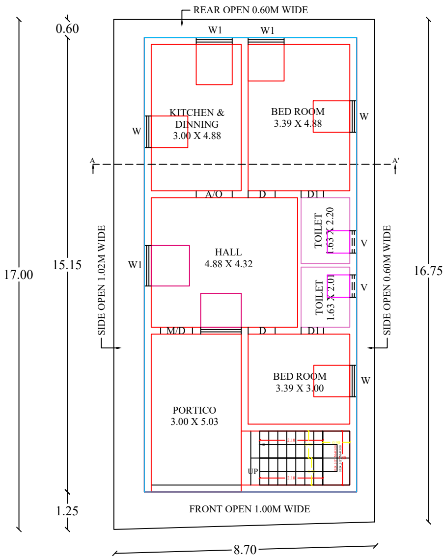
GROUND FLOOR PLAN (NORTH FACING)
