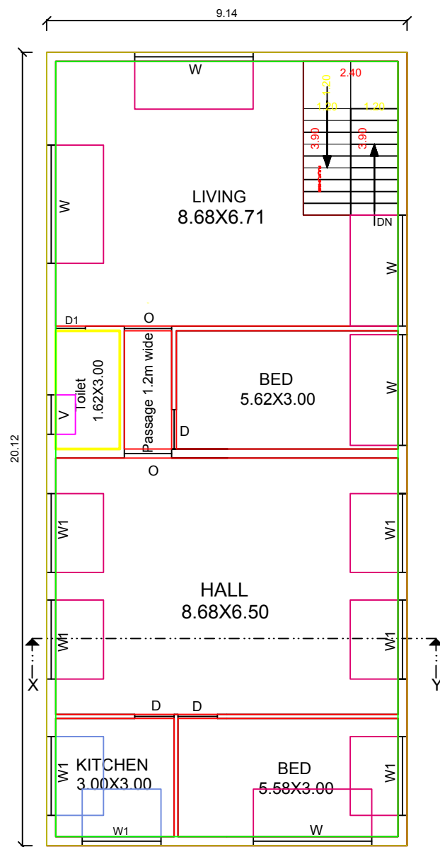
FIRST FLOOR PLAN FACING EAST (Residential)
