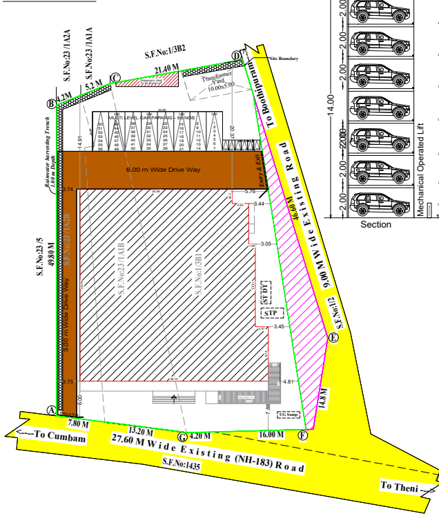
SITE PLAN
