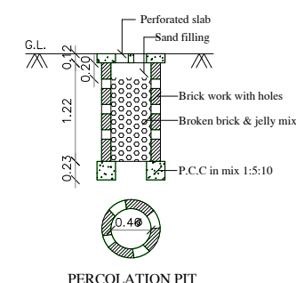
PERCOLATION PIT
