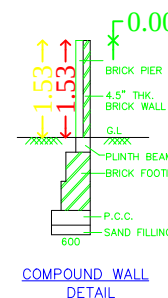
COMPOUND WALL DETAIL
