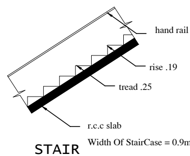
STAIR
