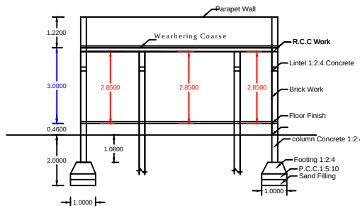
SECTION SECTION - AB
