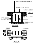
SEPTIC TANK DETAILS
