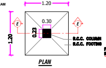
DETAILS OF COLUMN FOOTING
