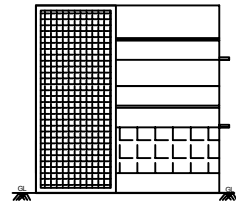
SECTION ON "A"
