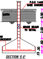
SECTION "E-E"
