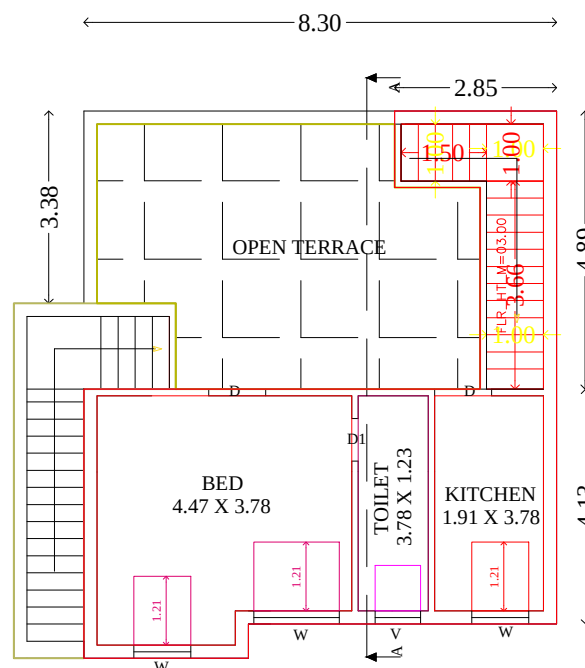
8.30 PROPOSED FIRST FLOOR (NORTH FACING)
