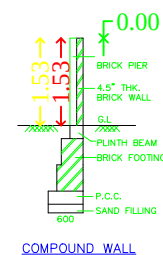
COMPOUND WALL
