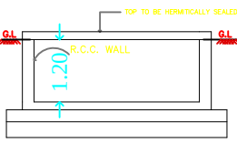
RWI SECTION (SAMPLE)
