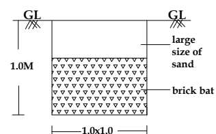
RAINWATER HARVESTING
