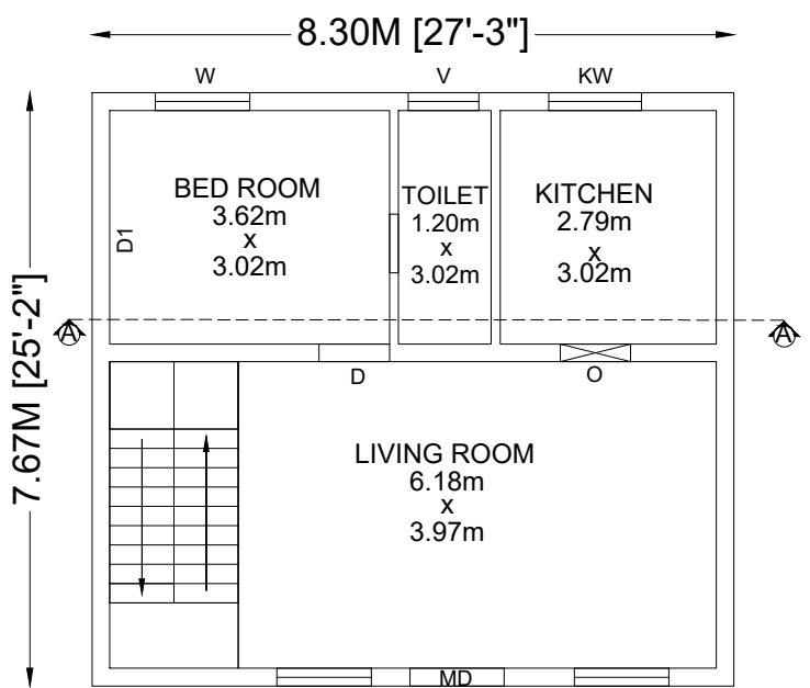
GROUND FLOOR PLAN (WEST FACING )
