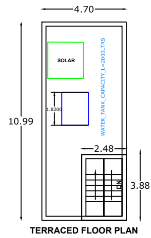
TERRACED FLOOR PLAN
