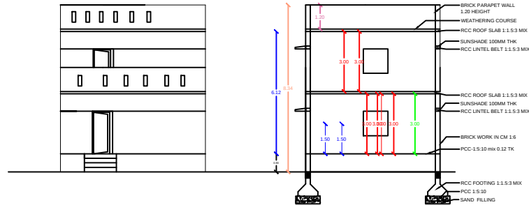
FRONT ELEVATION
