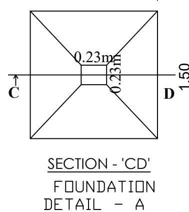
Isolated Footing -A (1.50X1.50) (Not to Scale)
