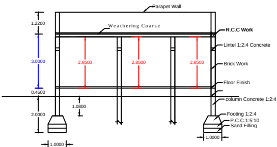
SECTION SECTION - AB
