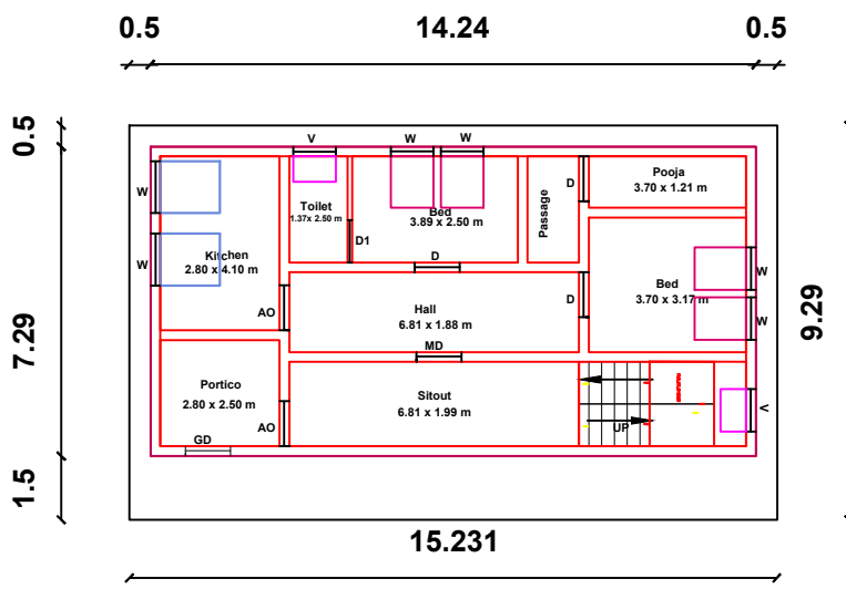
GROUND FLOOR PLAN (North Facing)
