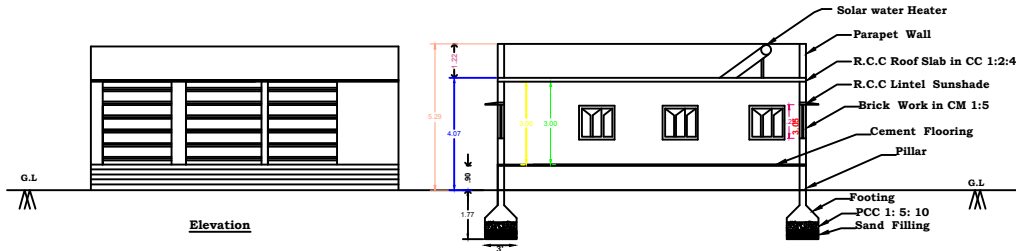
Section On XX
