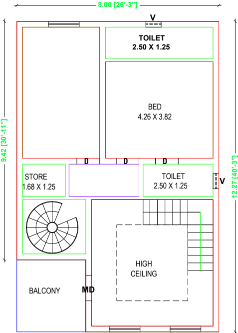
FIRST FLOOR PLAN [EAST FACING]
