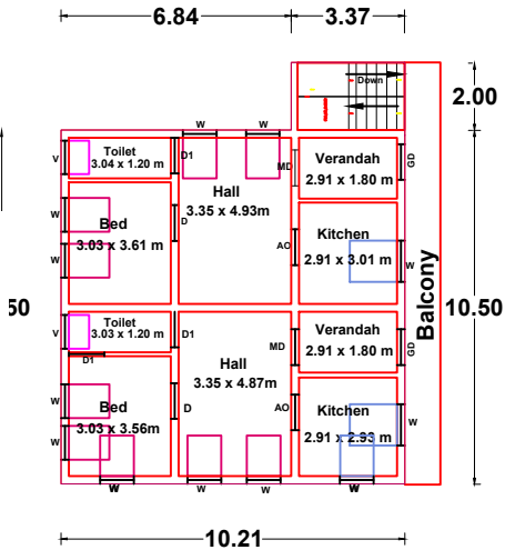
PROPOSED FIRST FLOOR (East Facing)
