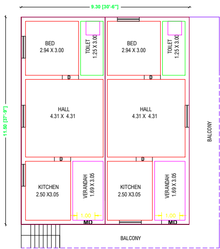
EX. FIRST FLOOR PLAN [EAST FACING]
