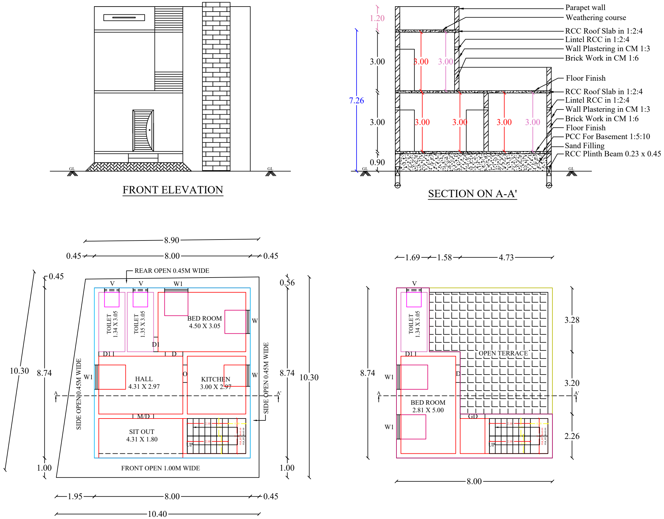
GROUND FLOOR PLAN (SOUTH FACING)
