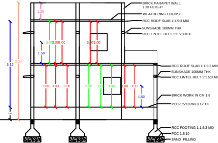
SECTION ON-AA
