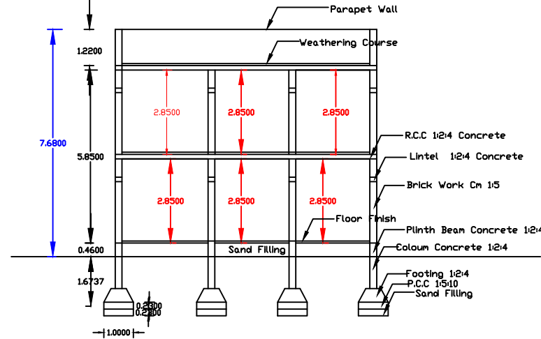
Section Section - AA
