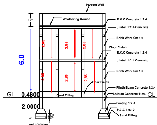
Section Section - AA
