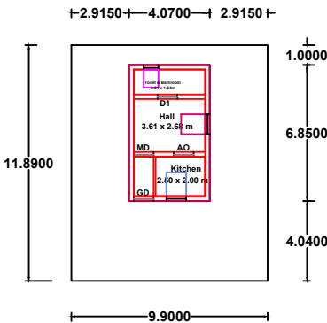
GROUND FLOOR (NORTH FACING)
