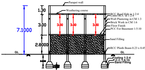
Section Section - AA
