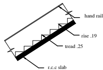
STAIR
