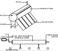
SOLAR HOT WATER SYSTEM DETAILS
