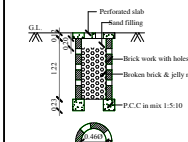
PERCOLATION PIT
