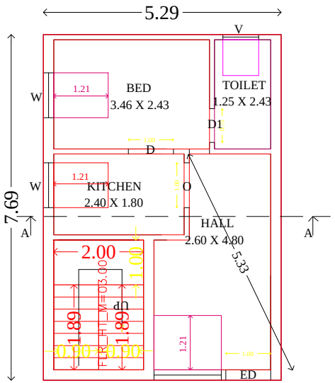
FIRST FLOOR (EAST FACING)
