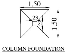
COLUMN FOUNDATION
