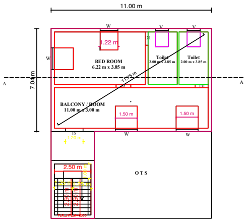
FIRST FLOOR PLAN [EAST FACING]
