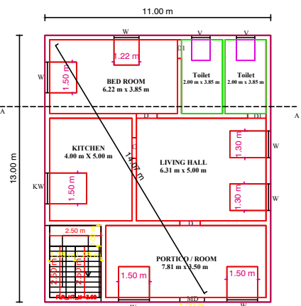
GROUND FLOOR PLAN [EAST FACING]
