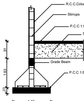
COLUMN DETAIL
