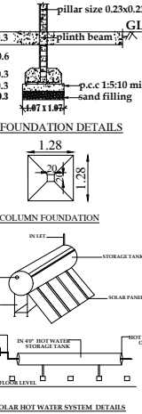
SOLAR HOT WATER SYSTEM DETAILS
