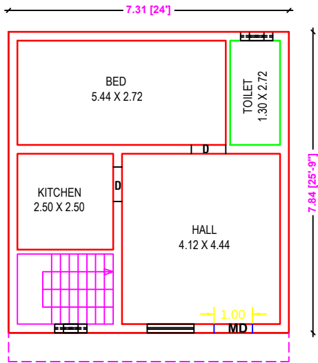
FIRST FLOOR PLAN [EAST FACING]
