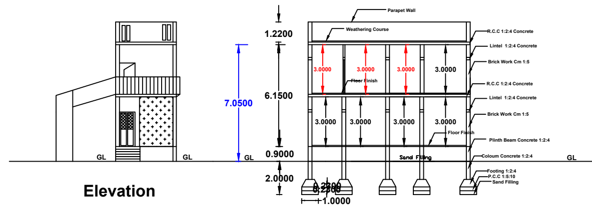
Section Section - AA
