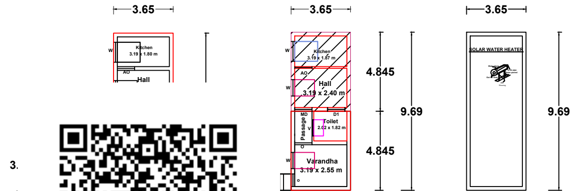
EXISTING FIRST FLOOR PROPOSED ADDITIONAL FIRST FLOOR
