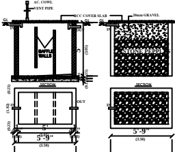
PLAN SEPTIC TANK
