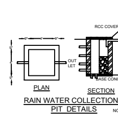
RAIN WATER COLLECTION PIT DETAILS
