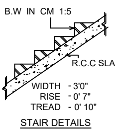
STAIR DETAILS
