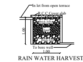
RAIN WATER HARVEST
