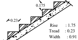
STAIRCASE DETAILS
